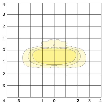
ISOFOOT CANDLE PLOT (TYPE II)
