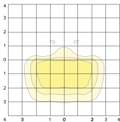
ISOFOOT CANDLE PLOT (TYPE IV)
