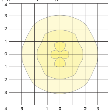
ISOFOOT CANDLE PLOT
