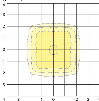
ISOFOOT CANDLE PLOT
