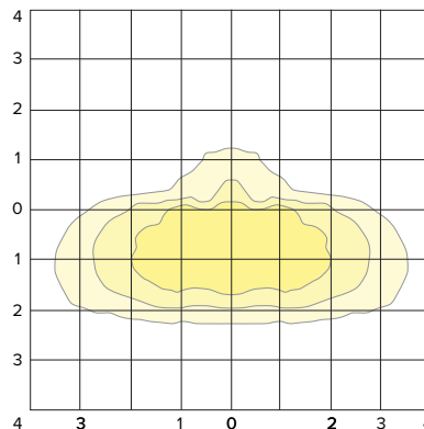
ISOFOOT CANDLE PLOT (TYPE III)
