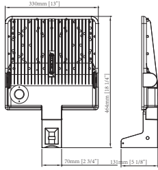
Arm mounting
